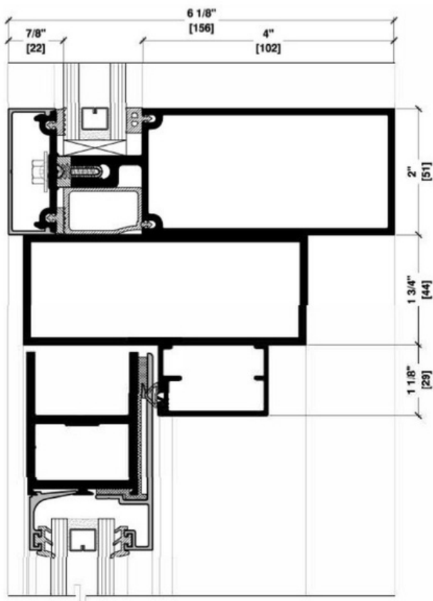
4' VERTICAL TUBE SERIES 175 DOOR HEAD CONDITION
